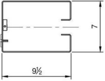
TRACK DETAIL 3:1
